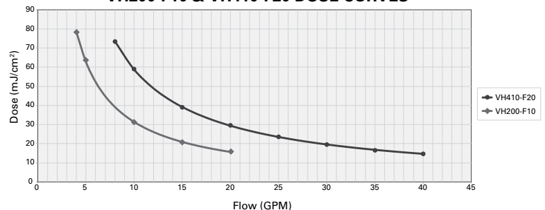
VH200-F10 & VH410-F20 DOSE CURVES
